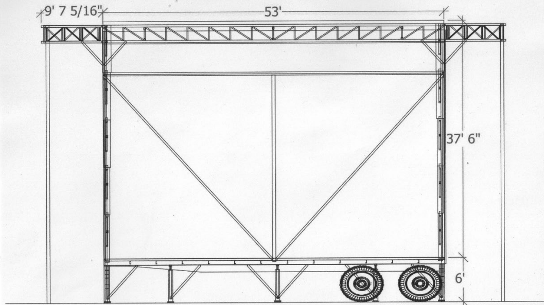
Front Elevation of Stage
