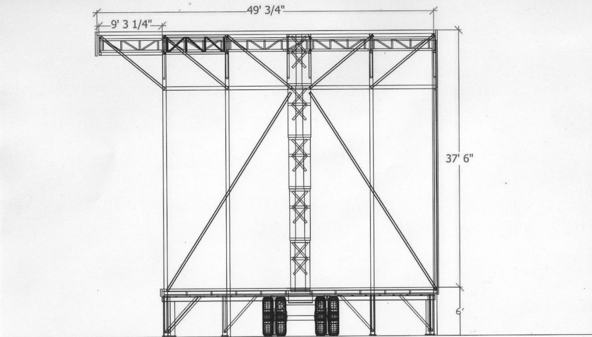
Right Side Elevation of Stage
